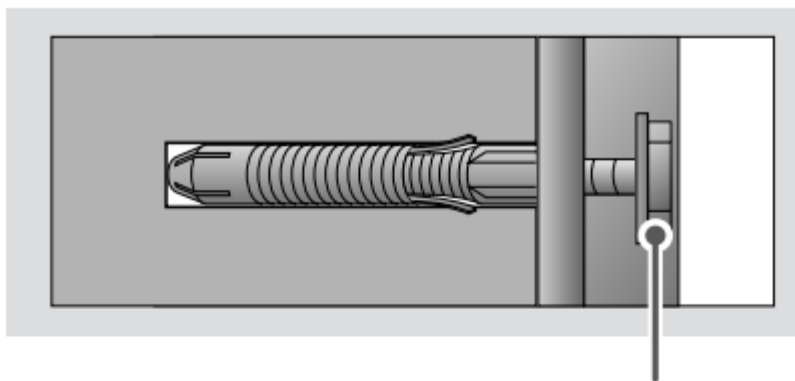
Wall mounting screw
