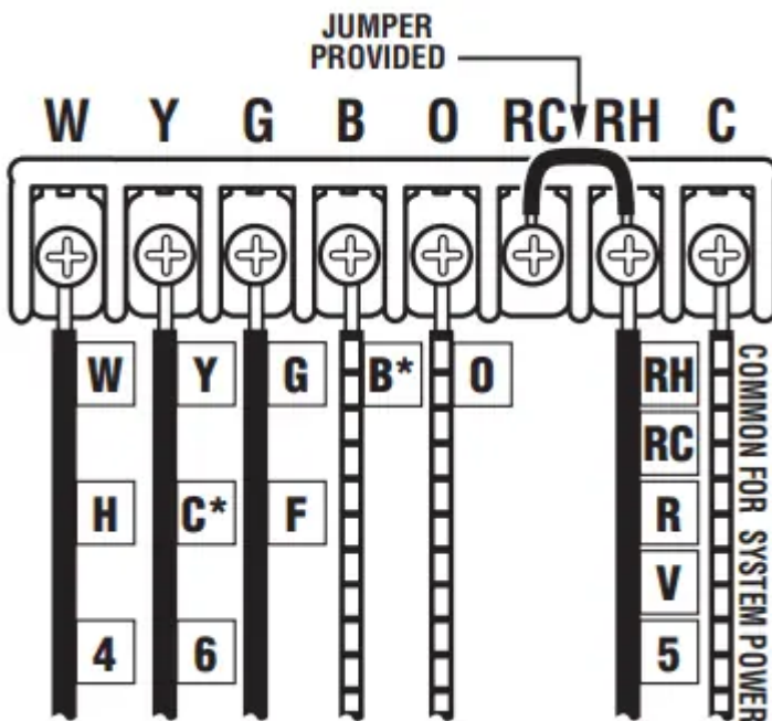
HEATING/COOLING SYSTEMS 4 + 5 Wire 1 Transformers
