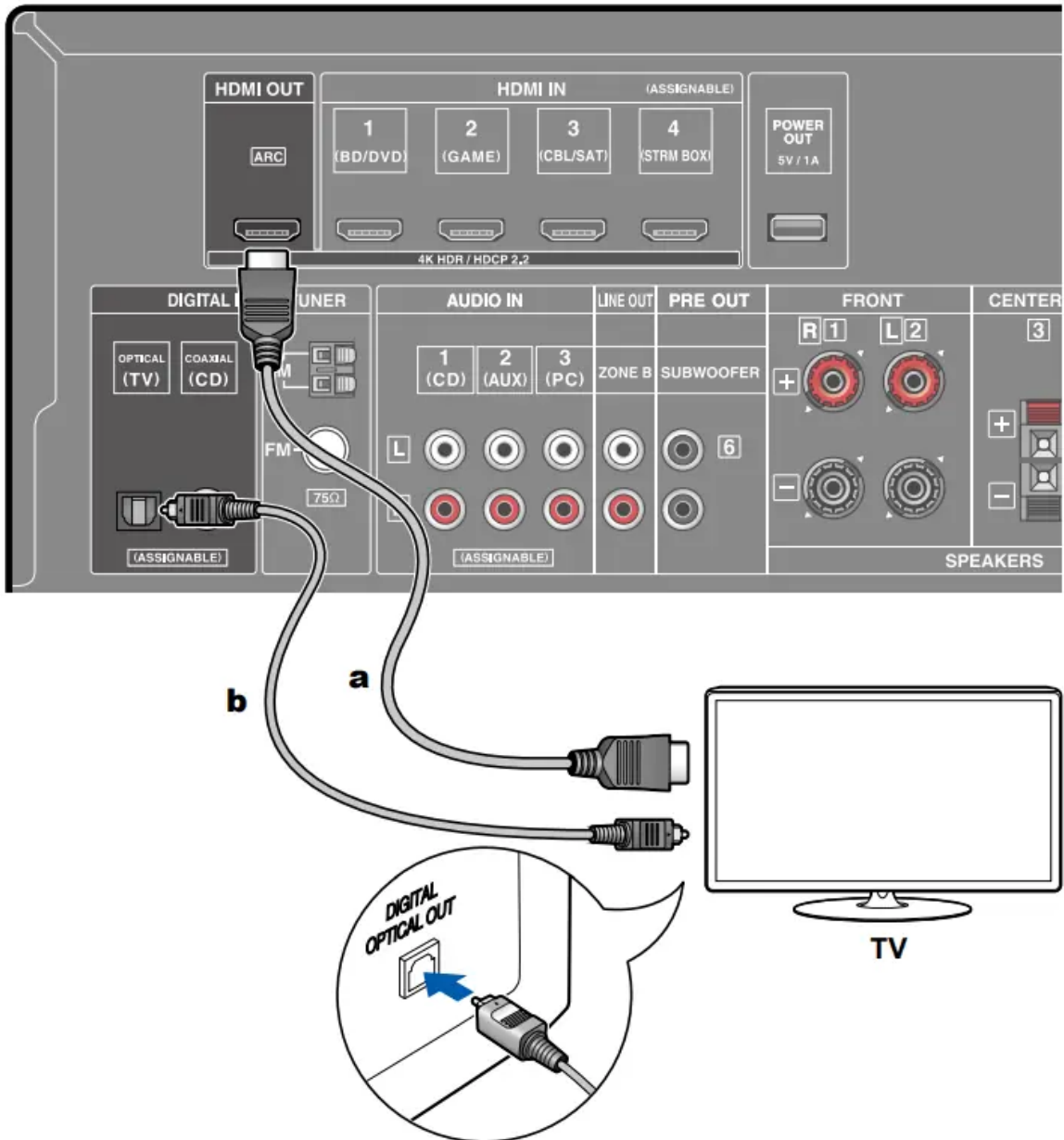
a HDMI cable, b Digital optical cable
