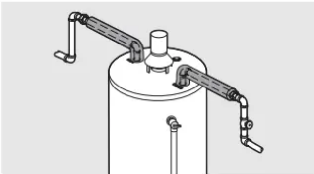
Typical horizontal piping arrangement
