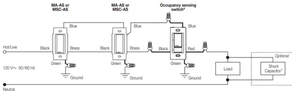
Wiring Diagram 17
