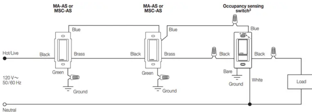
Wiring Diagram 11
