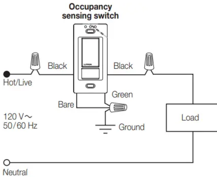
Wiring Diagram 2
