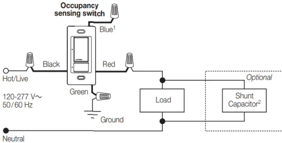
Wiring Diagram 14
