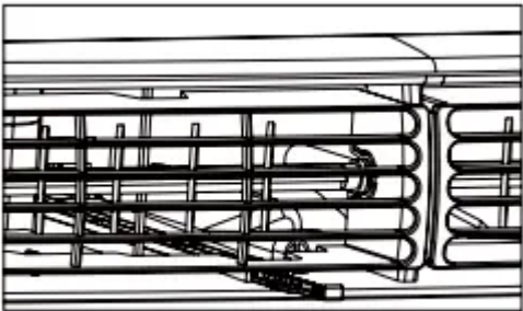
Figure 3 (VENT OPEN)
