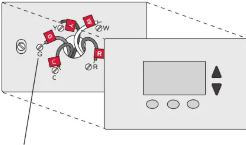
Terminal designation
