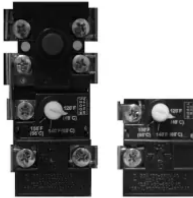
Figure 36 - Upper and Lower Thermostats
