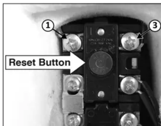
Figure 23 - Energy Cut Off (ECO) button
