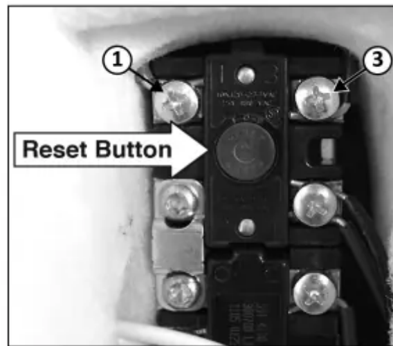
Energy Cut Off (ECO) button
