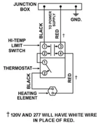
C-2 STANDARD SINGLE ELEMENT
