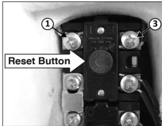
Figure 23 - Energy Cut Off (ECO) button
