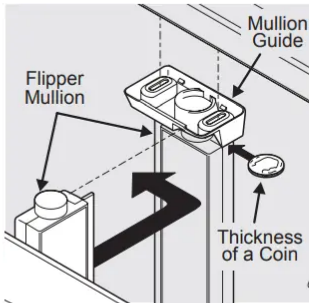
Adjusting Flipper Mullion Height
