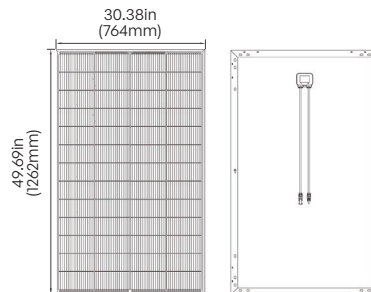
RSP200DC-ASR
