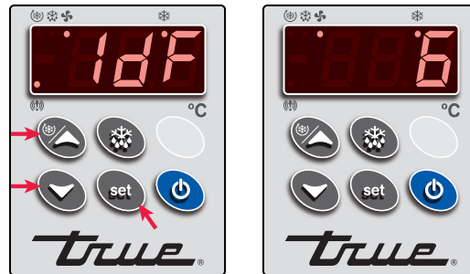
Dixell Control XW60VS
