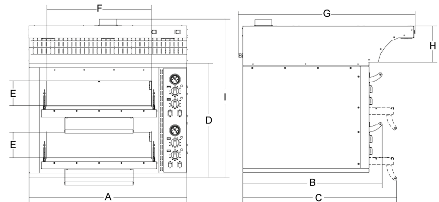
FIG. n°2 - Overall dimensions
