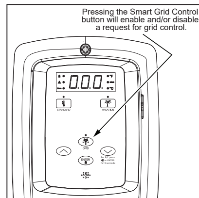
Figure 23 - Smart Grid Control Button
