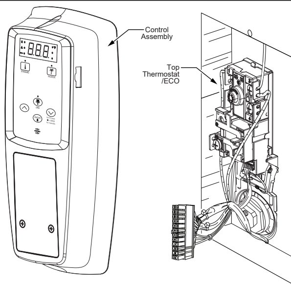
Figure 21 - Control Assembly
