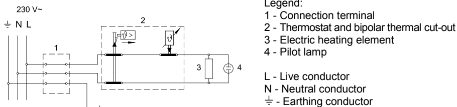
Electric installation
