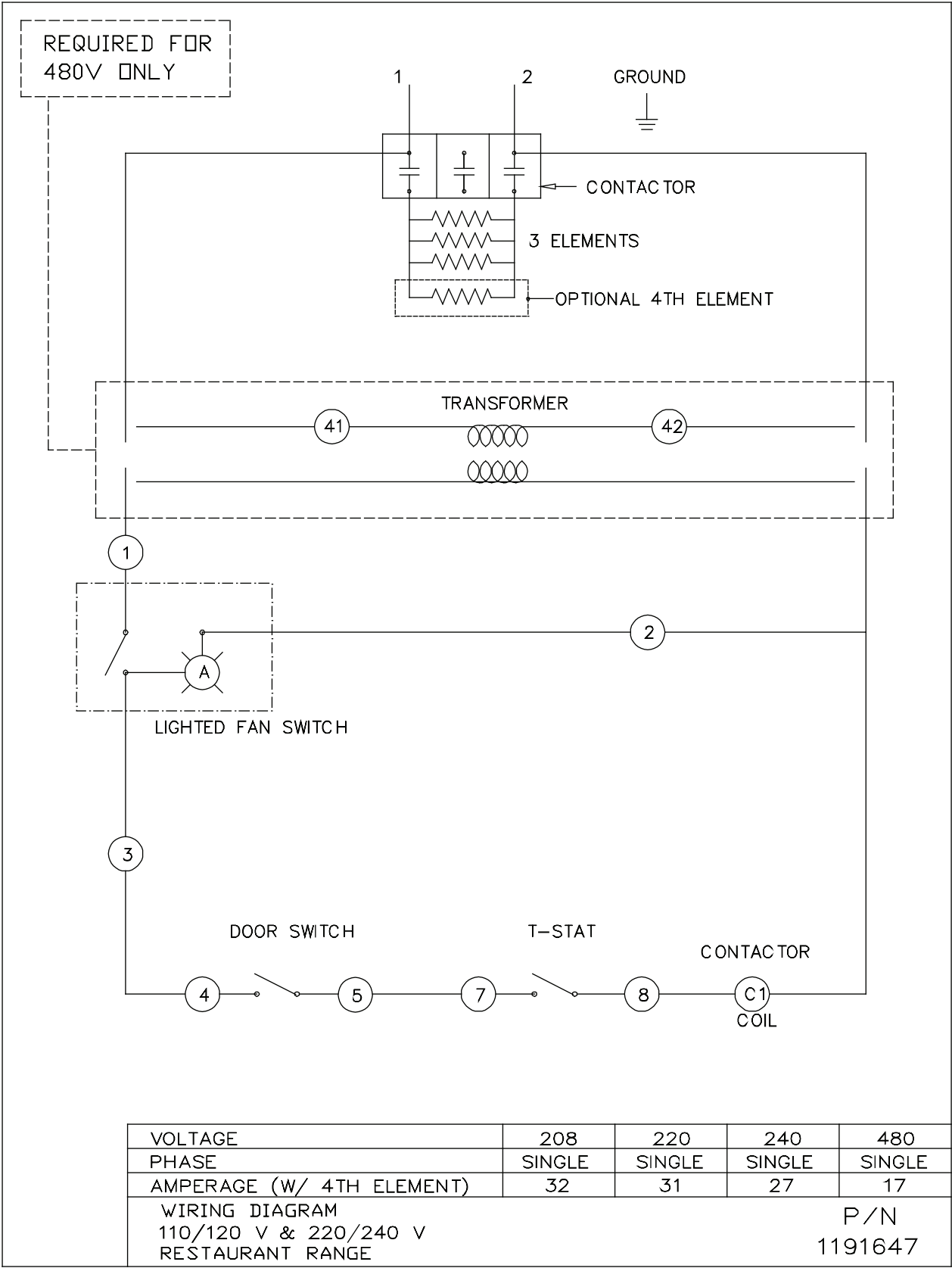
Figure 13 Wiring Diagram for Electric Standard Oven
