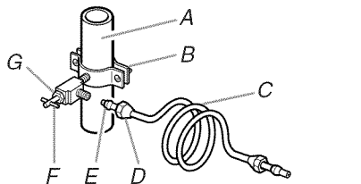
A. Cold water pipe B. Pipe clamp C. Copper tubing D. Compression nut E. Compression sleeve F. Shutoff valve G. Packing nut
