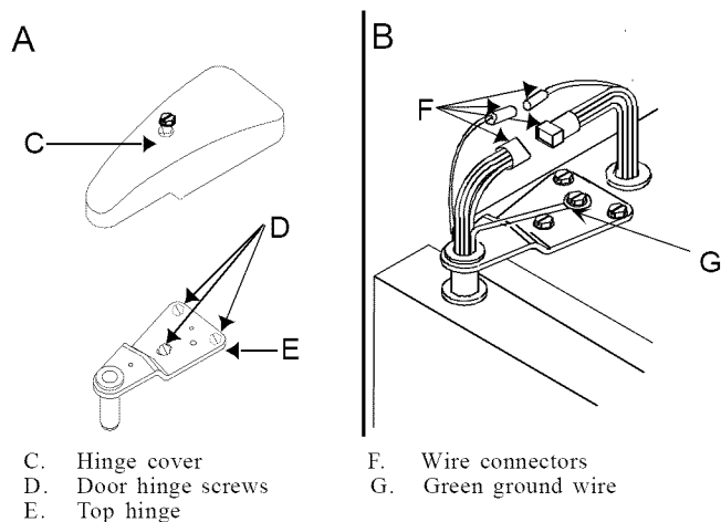
Top hinge removal
