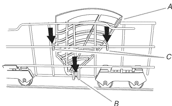
A. Top alignment B. Bottom slotted guide C. Knife holder hooks
