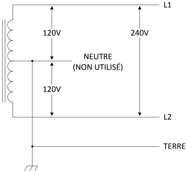
Figure 3 : Monophasé 220/240V
