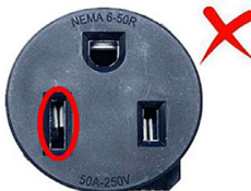
Figure 5. Example of a bad NEMA 6-50 receptacle
