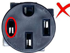
Figure 2. Example of a bad NEMA 14-50 receptacle
