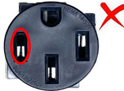
Figure 2. Example of a bad NEMA 14-50 receptacle
