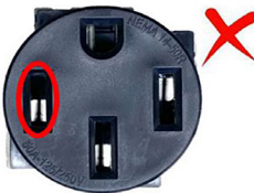
Figure 2. Example of a bad NEMA 14-50 receptacle
