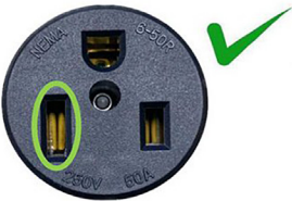
Figure 4. Example of a good NEMA 6-50 receptacle
