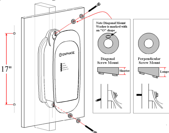
Figure 8: Mounting EVSE to a Hollow-Wall
