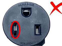
Figure 5. Example of a bad NEMA 6-50 receptacle
