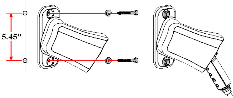
Figure 10: Mounting the SAE J1772 Connector Holster Using the Exterior Wood Screws and Washers
