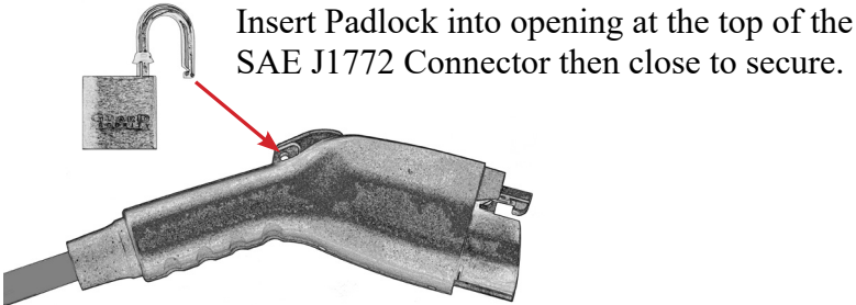
Figure 11: Locking the SAE J1772 Connector with Padlock Included
