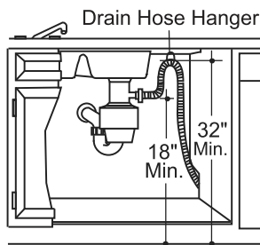
Disposer Installation
