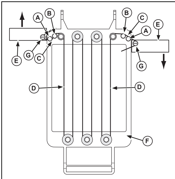
Figure 2. Replacing the Cutting Wire (3/4" Cut Model Shown).
