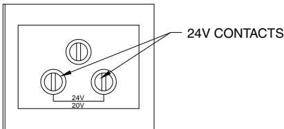
TRANSFORMER WIRING
