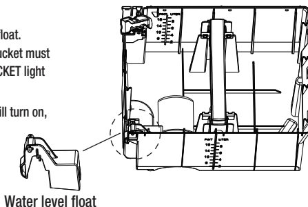
Water level float
