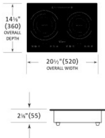
Overall Dimensions
