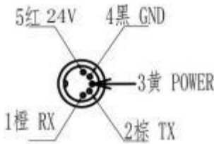
KP05-02 Interface Diagram
