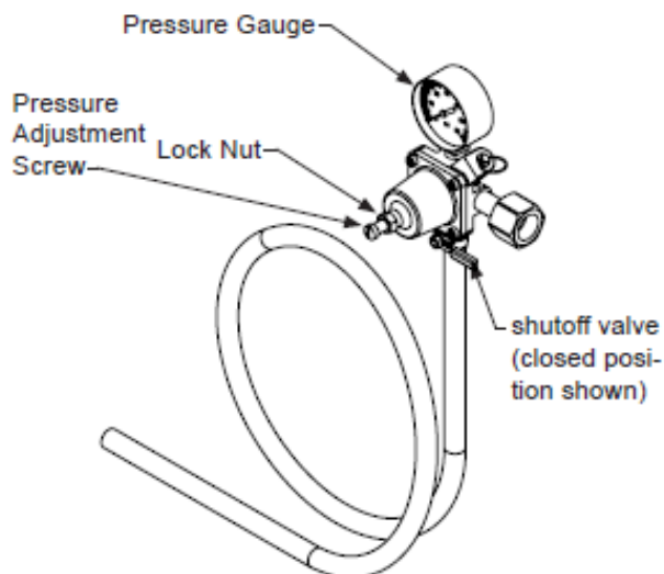
Figure 44 (Regulator for Single Dispense Tower)
