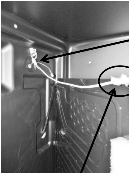
Defrost Sensor Location.
