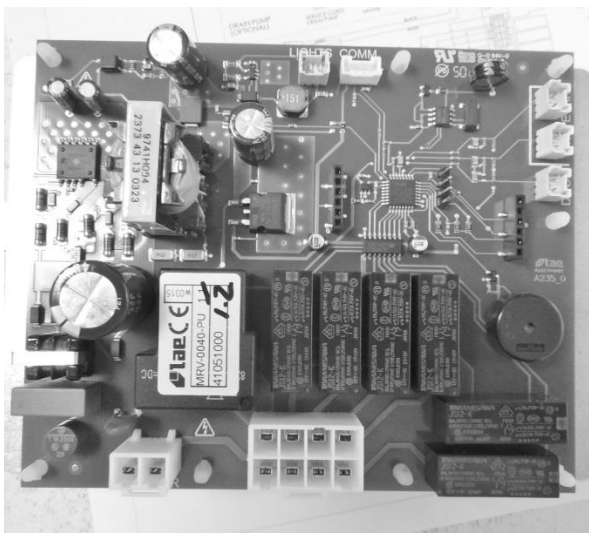
View of main power board. See wiring diagram and schematic included in this section.
