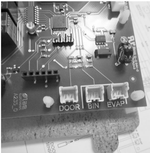
Connectors J3 – J5 (right to left): See wiring diagram and schematic included in this section.
