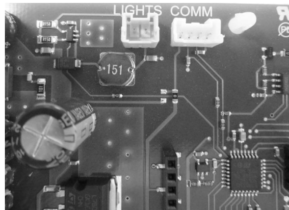
Connectors J6 & J7: (left to right): See wiring diagram and schematic included in this section.
