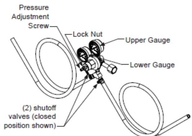
Figure 45 (Regulator for Double Dispense Tower)
