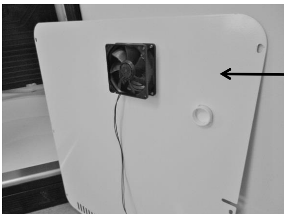
Evaporator fan is secured to the rear of the evaporator cover.
