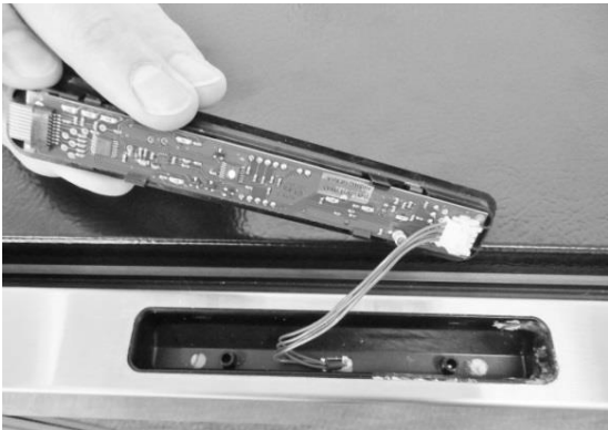
Lift user interface away from door receiver.
