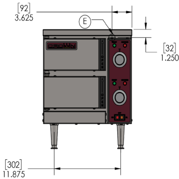
DIMENSIONS ARE IN INCHES [MM]
