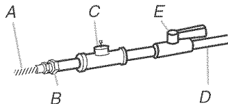
A. ¾" flexible gas connector B. ¾" pipe to flare adapter fitting C. ⅛" NPT minimum plugged tapping D. ½" NPT gas supply line E. Gas shutoff valve
