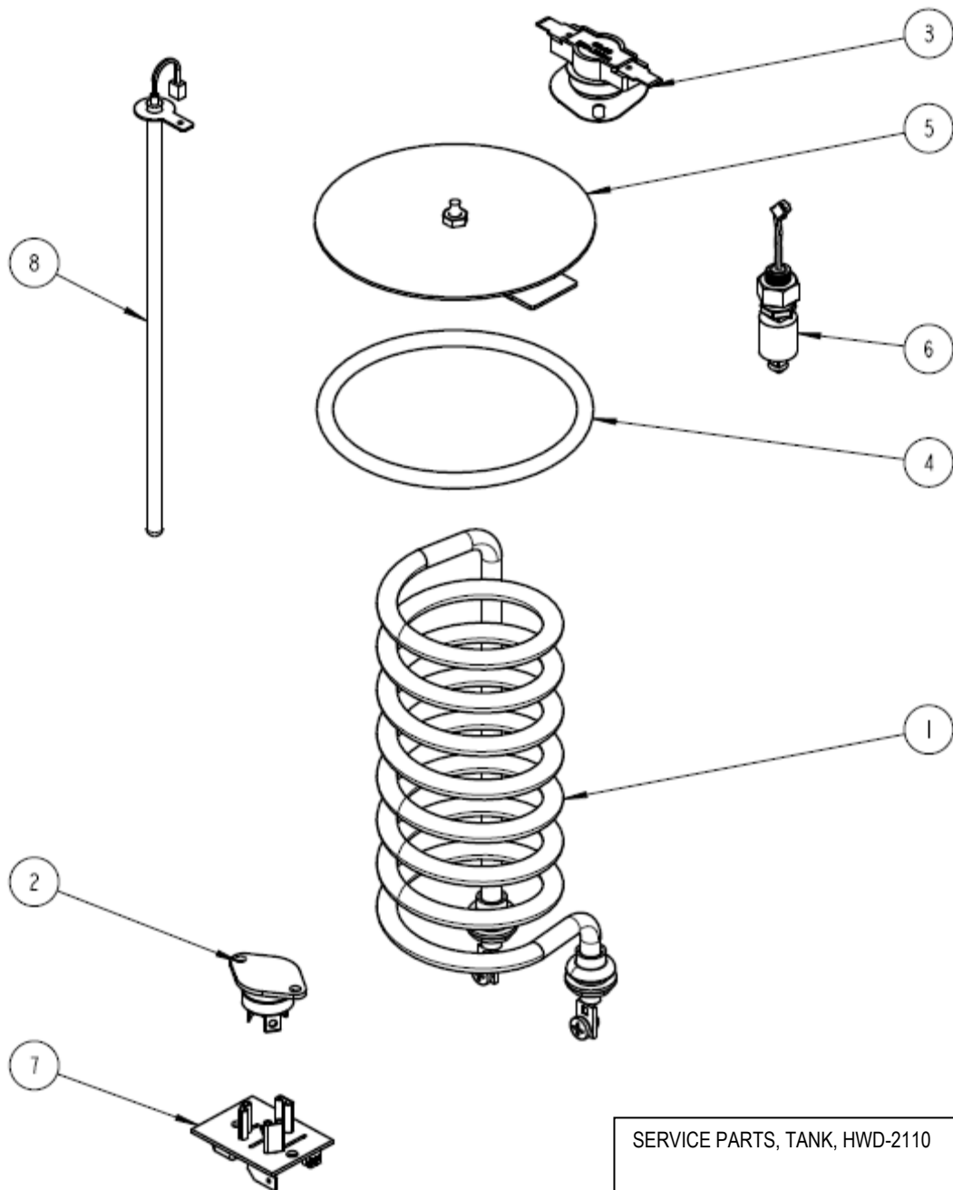
PARTS LIST FOR HWD-2110 Hot Water Tank Drawing 1104.00028.00
