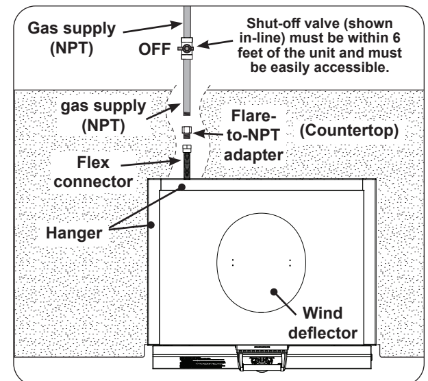
Fig. 29-2 Household LP & Nat. gas diagram
