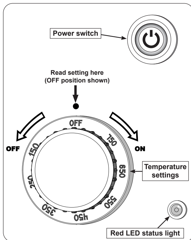
Fig. 35-1 Ignition components
