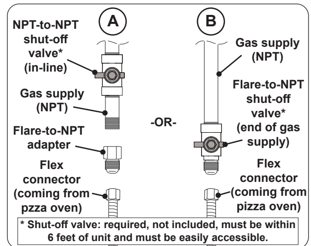
Fig. 29-1 Connecting to a gas line
