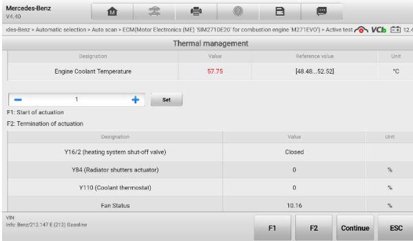
Figure 4-14 Active Test Screen
