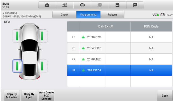
Figure 5-5 Copy by Activation Function Main Screen
