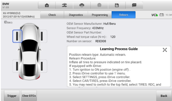
Figure 5-8 Relearn Function Main Screen
