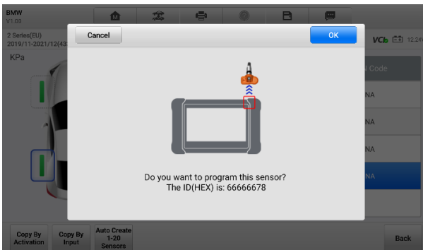
Figure 5-6 Copy by Activation Function Screen
