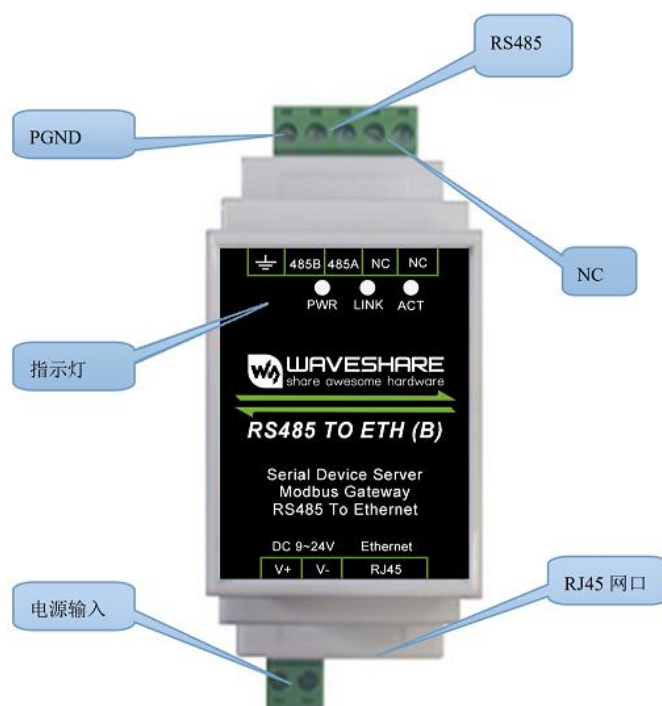
Figure 3 Front view
