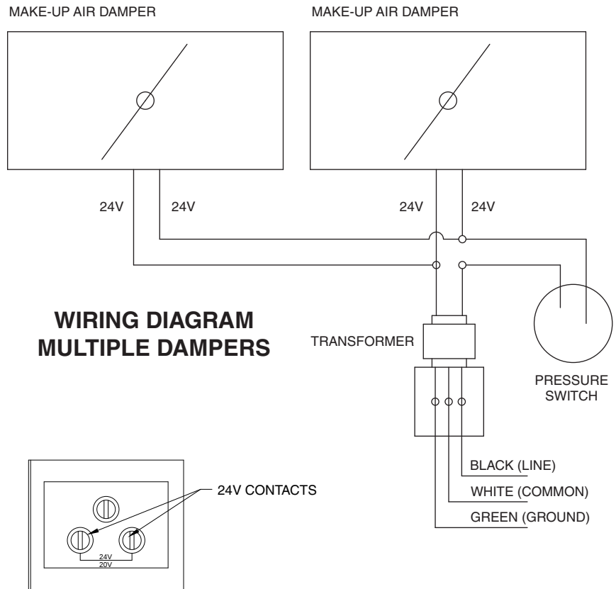
TRANSFORMER WIRING
