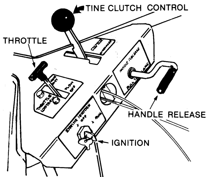
FIG. 2--PANEL CONTROLS
