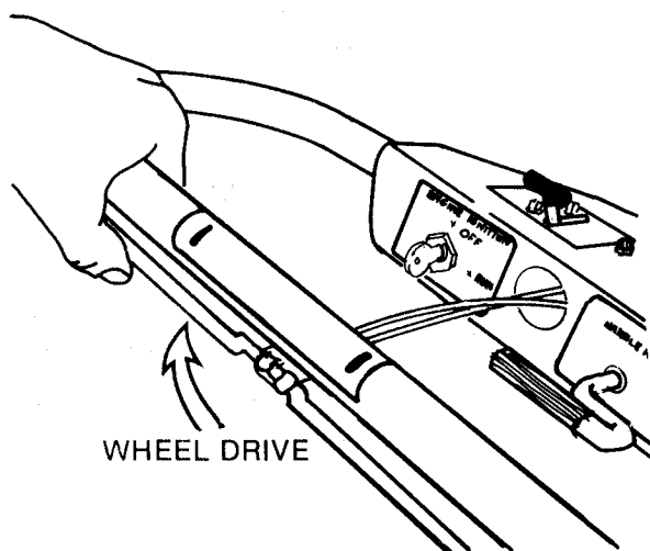
FIG. 3--CLUTCH CONTROL
