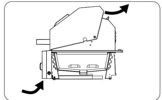
Fig. 32-1 Airflow diagram
