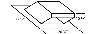
LOW PROFILE ROOF JACK (MAXIMUM 4/12 PITCH)
