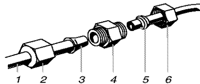
1. Line to refrigerator 4. Coupling (purchased) 2. Nut (provided) 5. Ferrule (purchased) 3. Bulb 6. Nut (purchased)
