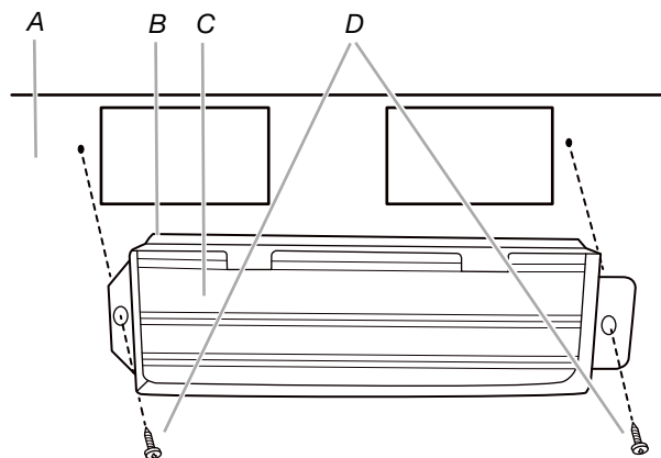
A. Back of microwave oven B. Damper assembly C. Damper blade D. Sheet metal screw 5/32" x 5/16" (4 mm x 8 mm)
