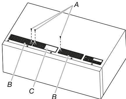
A. Screw B. Recirculation vent covers C. Recirculation lighting cover
