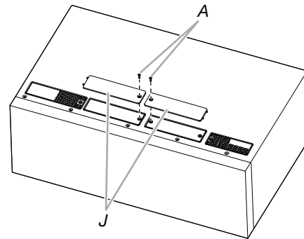
A. Screws J. Exhaust vent covers
