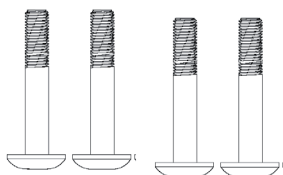
Vis Allen M8*40*20
