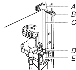
A. Tube clamp B. Tube clamp screw C. Plastic tubing D. Compression nut E. Valve inlet
