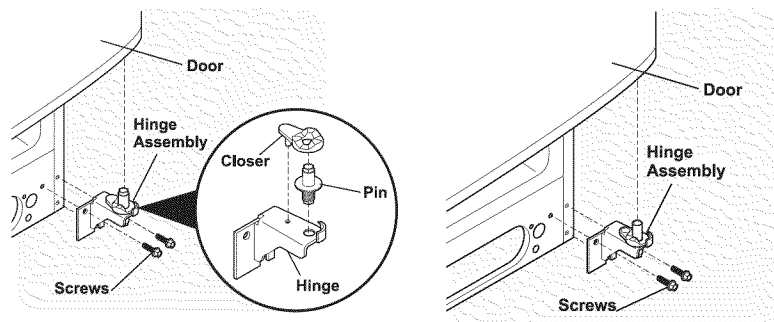
Adjustable Hinge (some models)
