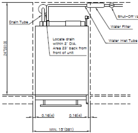
Fig. 4 Top View
