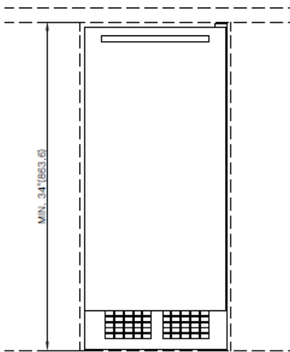
Fig. 5 Front View
