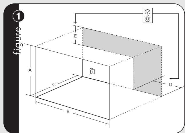
Surface Mount Cutout Dimensions
