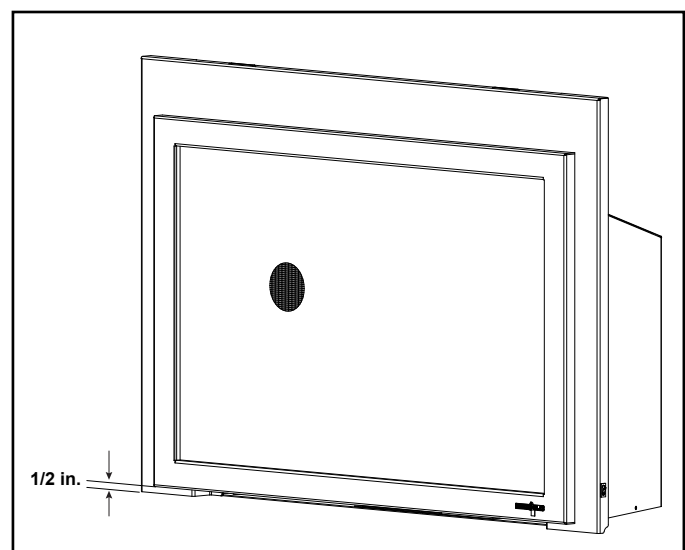
Figure 3.9 Minimum Required 1/2 in. Gap
