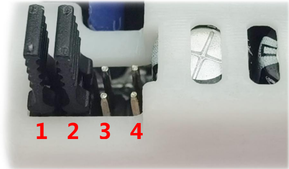
Insert jumper cap 1, 2
