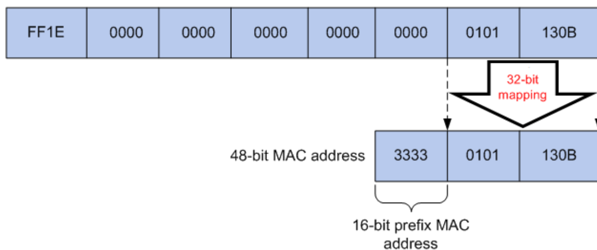
Figure 8-3 Mapping relationship between multicast IPv6 address and multicast IPv6 MAC address
