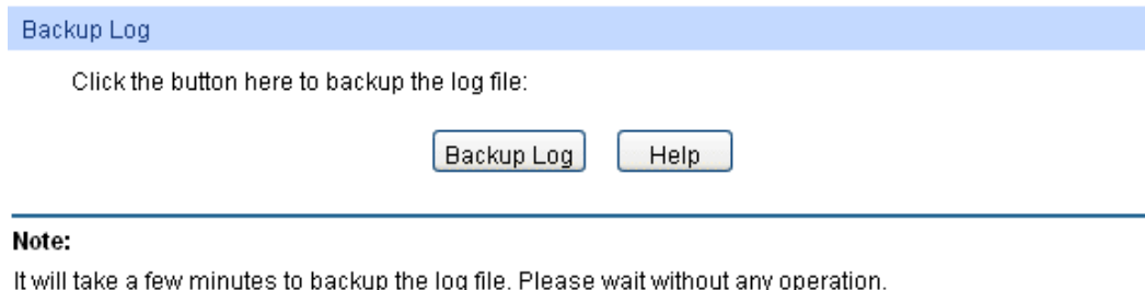
Figure 14-6 Backup Log
