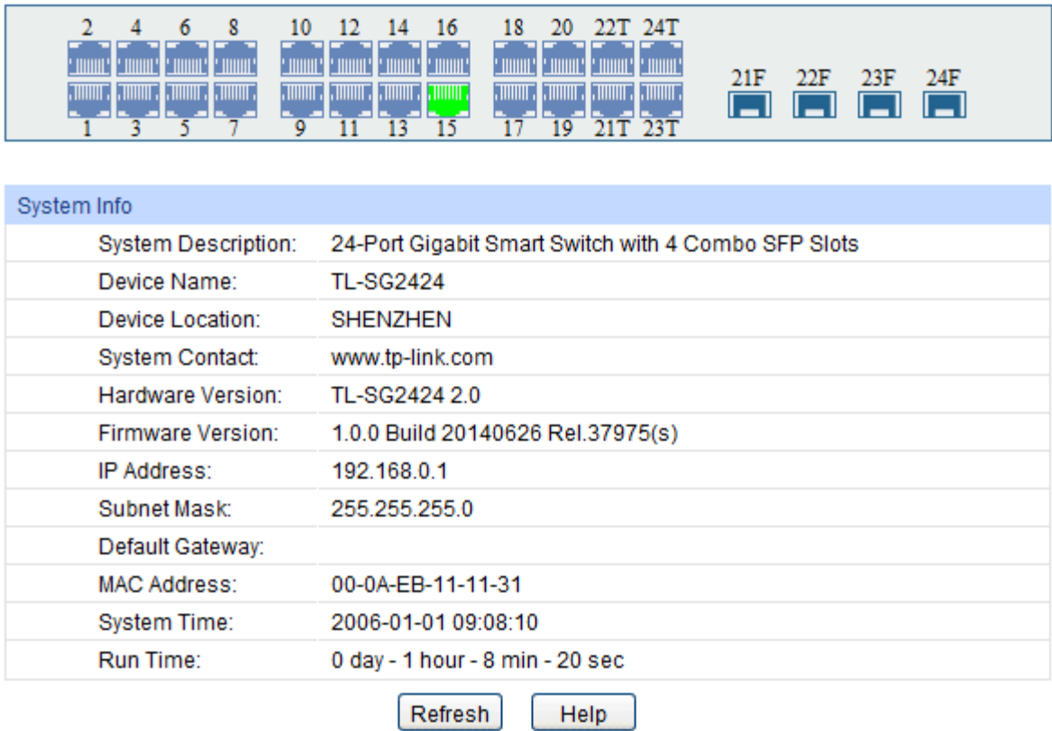
Figure 4-1 System Summary
