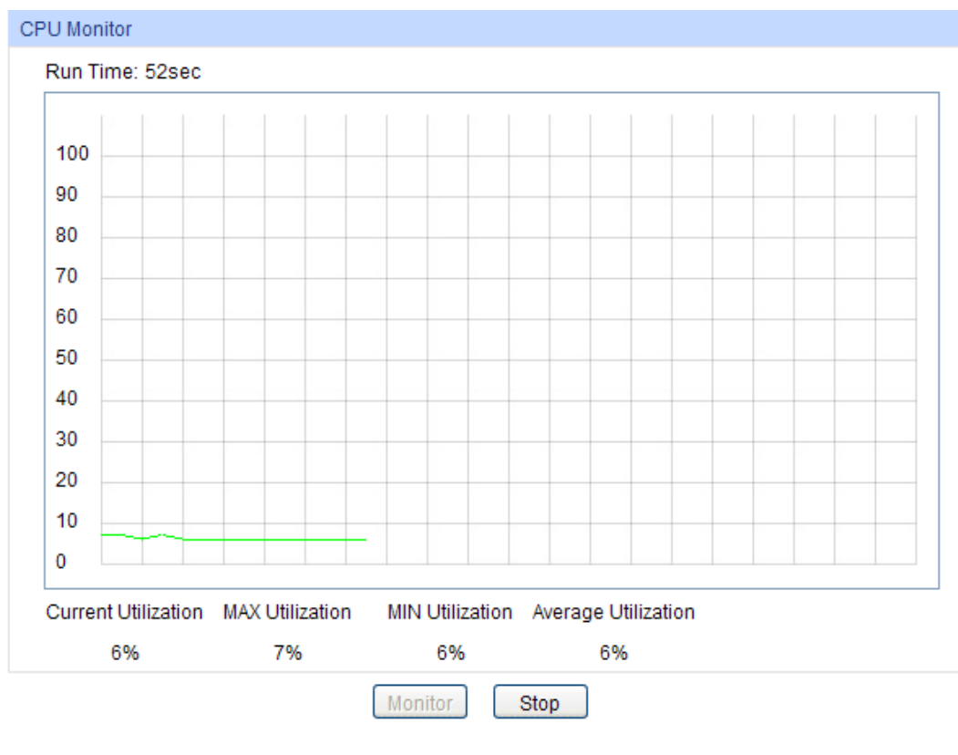
Figure 14-1 CPU Monitor
