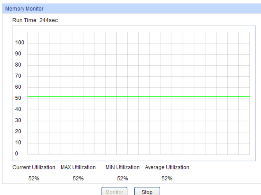
Figure 14-2 Memory Monitor
