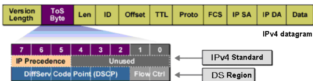
Figure 9-3 IP datagram
