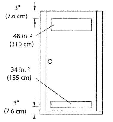
Closet Door Clearance Requirements
